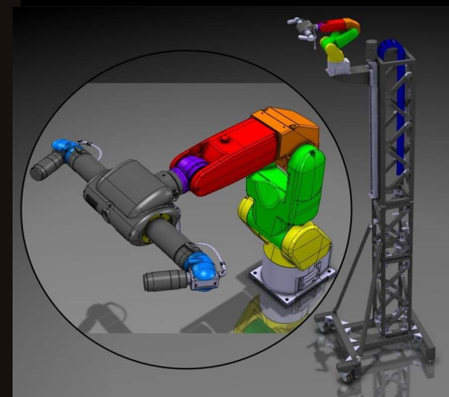
3D geometry acquisition – custom made measurement systems
